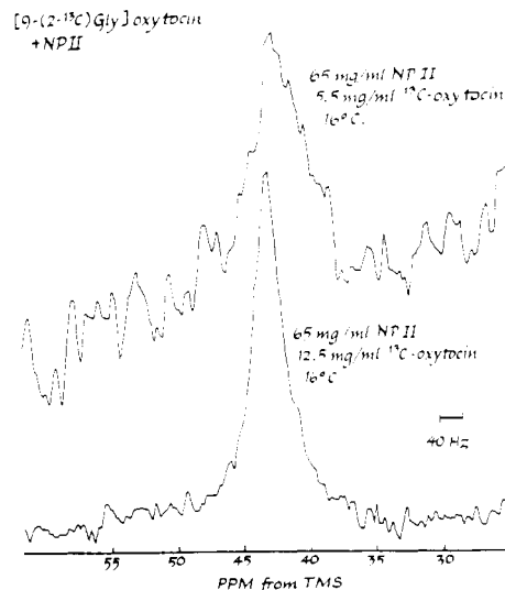
FIGURE 5: Spectra of NPII, 65 mg/mL, 16 °C, + [9-[2- 13 C]glycinamide]oxytocin. (Top) Hormone:protein ratio is 0.85:1.0; (bottom) hormone:protein ratio is 1.9:1.0. Spectra taken at 22.6 MHz on WH-90 spectrometer. Total accumulation time (0.2-s repetition rate, 90° pulses) for each spectrum was about 6 h.
