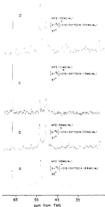
FIGURE 4: Spectra of NPI and NPII + [1-hemi-L-[2- 13 C]cystine]oxytocin at hormone:protein ratios of about 1.4:1.0. (a) NPI, 65 mg/mL, 22 °C; (b) NPI, 25 mg/mL, 37 °C; (c) NPI, 11 mg/mL, 37 °C; (d) NPII, 25 mg/mL, 37 °C.
