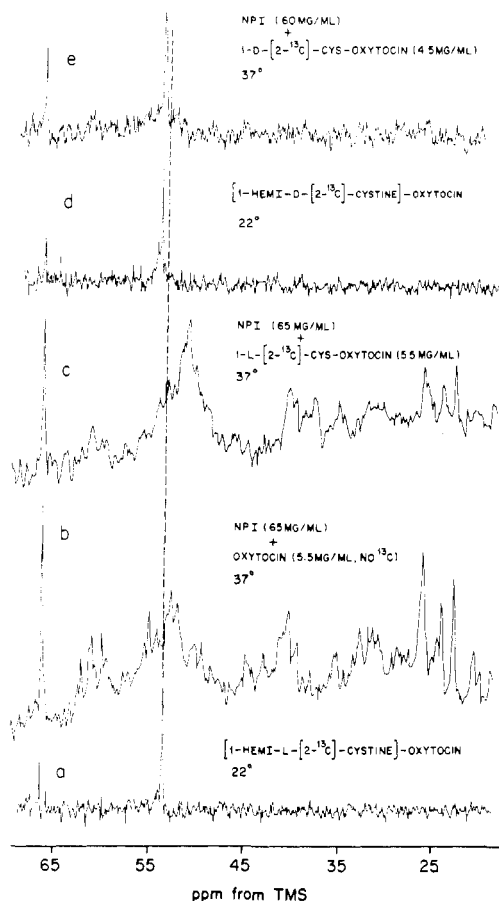
FIGURE 1: ^{13}\text{C} NMR spectra of (a) [1-hemi-L-[2- ^{13}\text{C} ]cystine]oxytocin (no neurophysin); (b) neurophysin I (NPI) + oxytocin (no enrichment; hormone:protein ratio is 0.9:1.0); (c) NPI + [1-hemi-L-[2- ^{13}\text{C} ]cystine]oxytocin (hormone:protein ratio as in b); (d) [1-hemi-D-[2- ^{13}\text{C} ]cystine]oxytocin (no neurophysin); (e) NPI + [1-hemi-D-[2- ^{13}\text{C} ]cystine]oxytocin (hormone:protein ratio is 0.75:1.0). All spectra measured at 67.9 MHz on a Bruker HX-270 spectrometer, with a solution pH of 6.6 \pm 0.1 (direct meter reading in \text{D}_2\text{O} ). The total accumulation time, using a 1-s repetition rate and 90^\circ pulses, for spectra a, d, and e was 10–20 min, while for b and c the accumulation time was 3–4 h. Spectrum b is displayed at about twice the amplitude of spectrum c. The sharp peak at 66.5 ppm is due to dioxane ( 2 \mu\text{L}/\text{mL} ).
