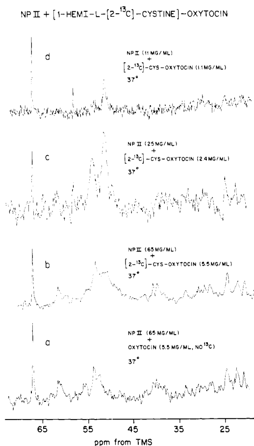
FIGURE 3: Spectra of NPII + oxytocin at hormone:protein ratios of about 0.9:1.0. (a) NPII (65 mg/mL) + oxytocin (no enrichment), 37 °C; (b-d) NPII + [1-hemi-L-[2- 13 C]cystine]oxytocin; (b) 65 mg/mL, 37 °C; (c) 25 mg/mL, 37 °C; (d) 11 mg/mL, 37 °C. Accumulation times were 3–6 h.
