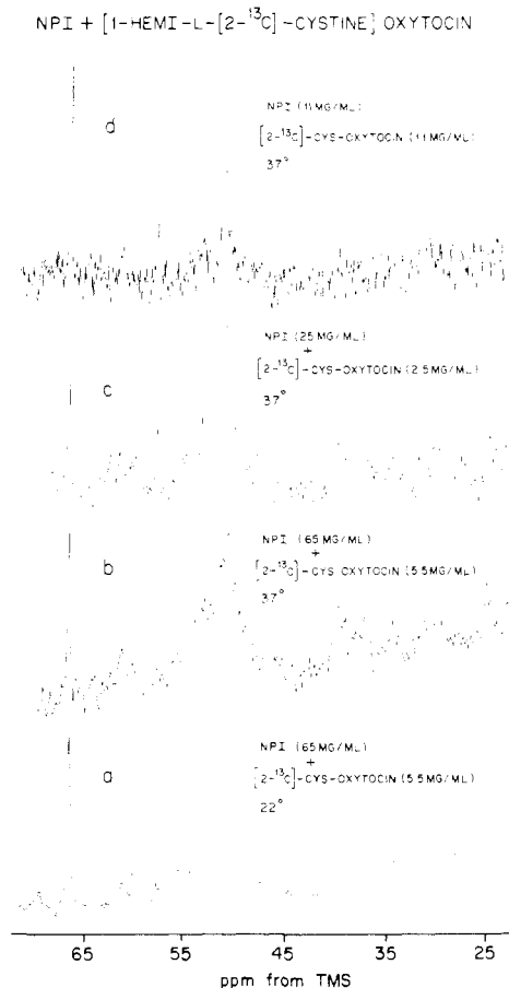
FIGURE 2: Spectra of NPI + [1-hemi-L-[2- ^{13}\text{C} ]cystine]oxytocin at hormone:protein ratios of about 0.9:1.0. Protein concentrations and temperatures are as follows: (a) 65 mg/mL, 22 °C; (b) 65 mg/mL, 37 °C; (c) 25 mg/mL, 37 °C; (d) 11 mg/mL, 37 °C. Spectral and solution conditions as in Figure 1. Accumulation times were 3–6 h. The peak in d at 57.5 ppm is due to EDTA (see text).
